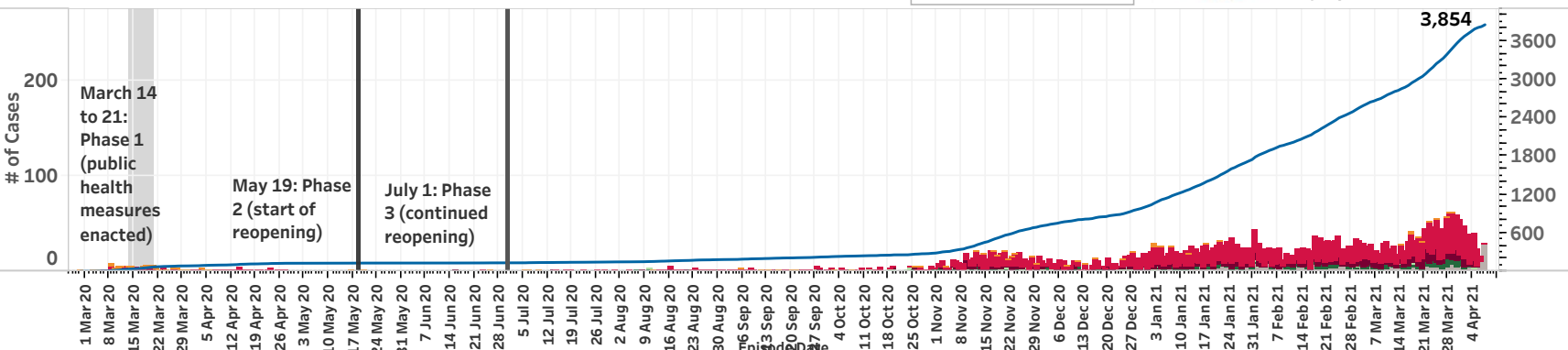
Graph 1: Exposure history of COVID-19 cases by Episode Date* (n=3,854)**
